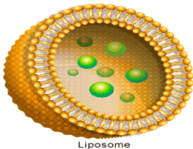
Figure 3: Schematic representation of a liposome [50]
